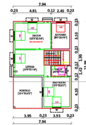
PROPOSED GROUND FLOOR PLAN
