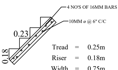
STAIRCASE DETAILS
