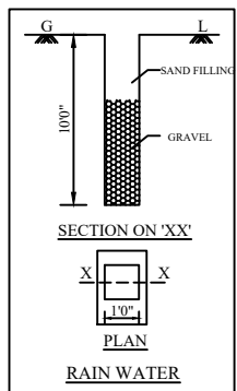
RAINWATER HARVESTING
