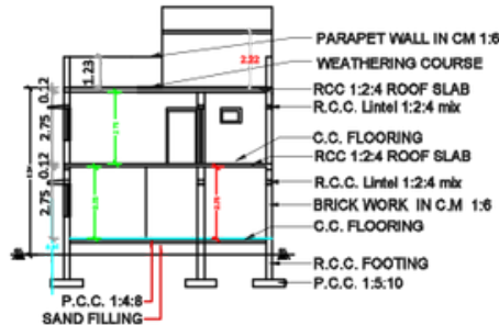
SECTION ON A-A (PROPOSED)
