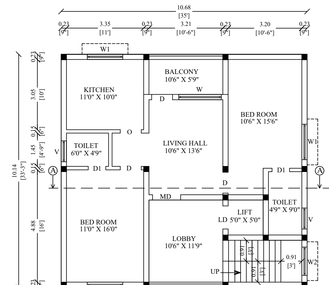
TYPICAL FIRST, SECOND & THIRD FLOOR PLAN
