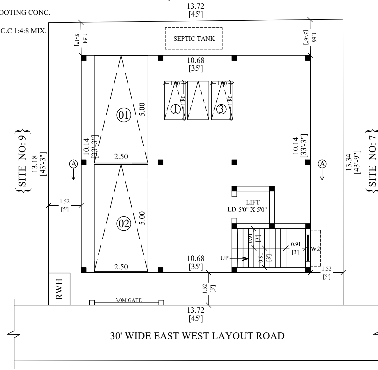
SITE PLAN & STILT FLOOR PLAN
