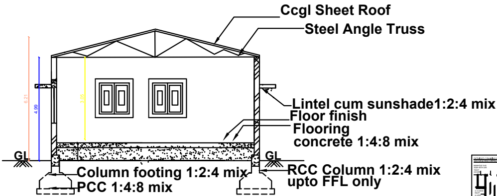
SECTION ELEVATION
