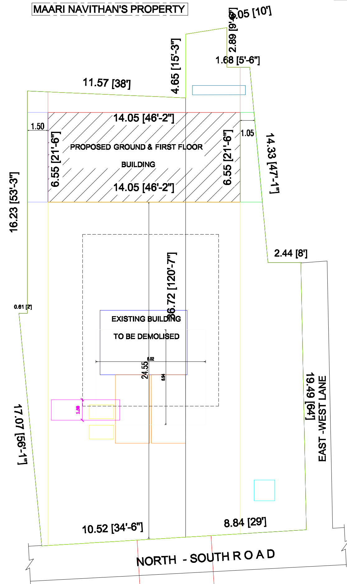
SITE PLAN
