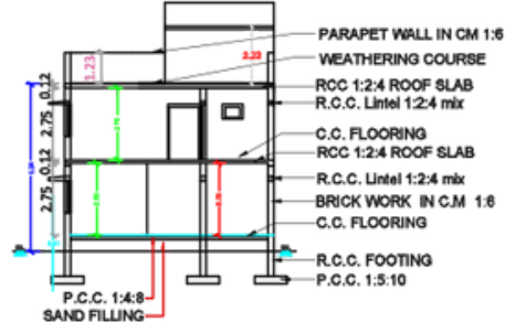
SECTION ON A-A (PROPOSED)
