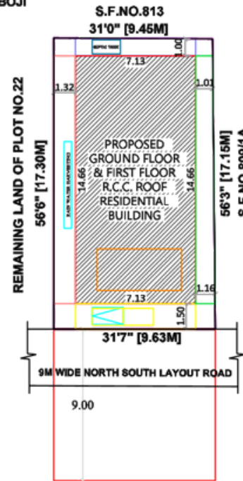
SITE PLAN (PROPOSED)
