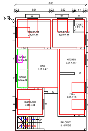
PROPOSED ADDITIONAL FIRST FLOOR BUILDING
