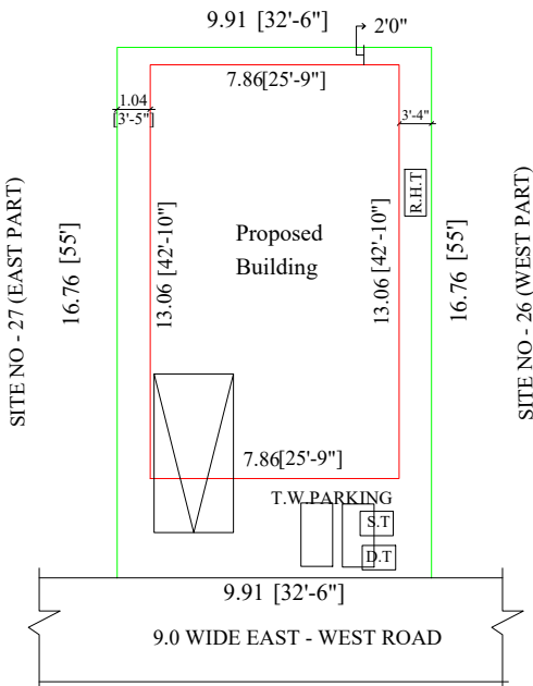
SITE PLAN
