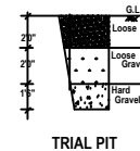
TRIAL PIT
