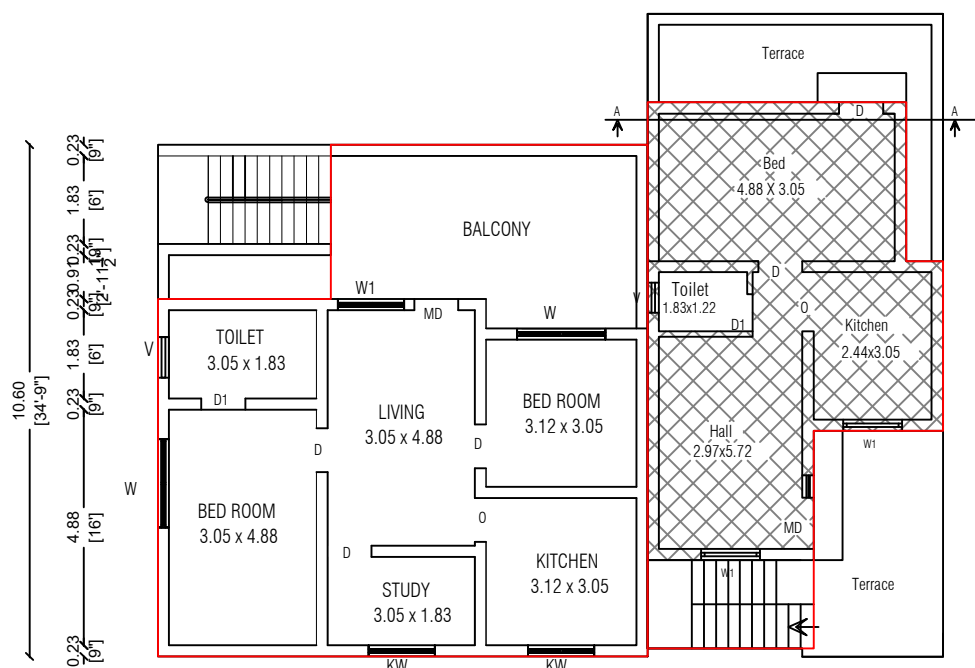
EXISTING & ADD. PROPOSED FIRST FLOOR
