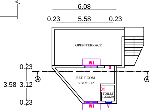
ADD. PROPOSED FIRST FLOOR
