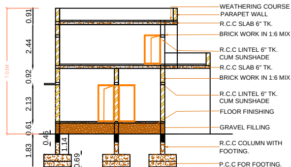
CROSS SECTION AT A-A
