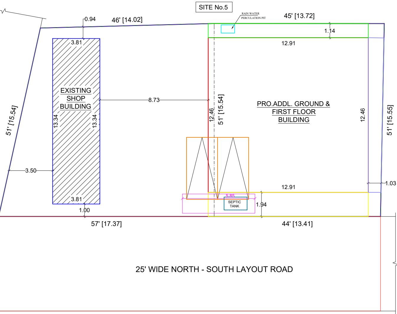
SITE PLAN
