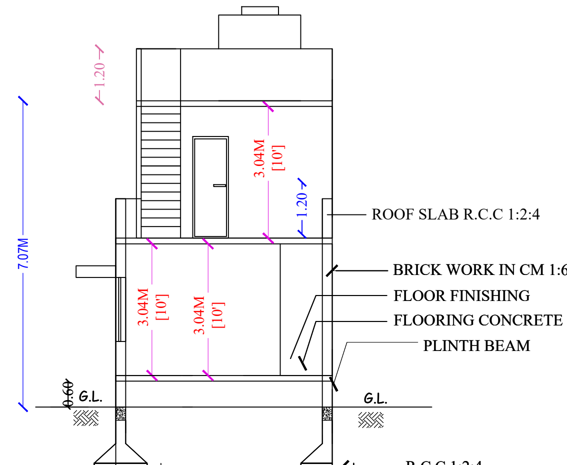
SECTION "A-A"
