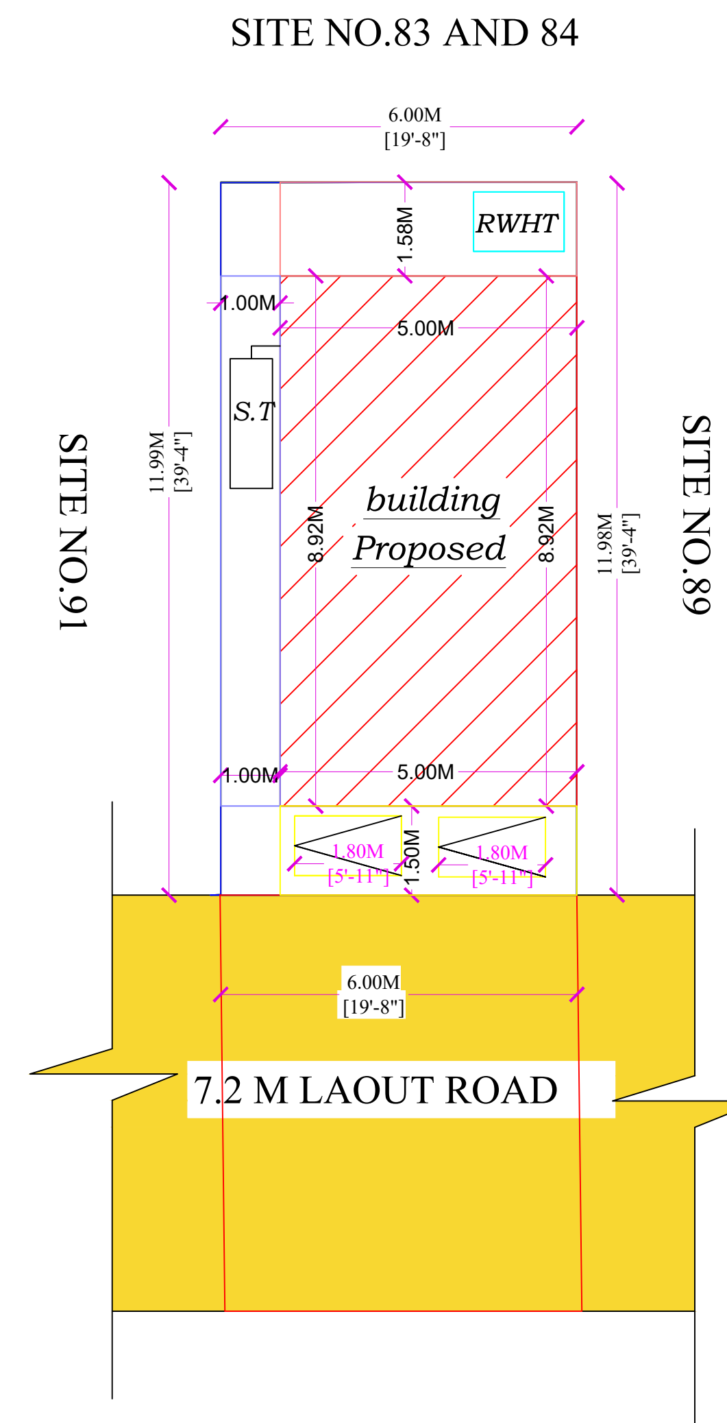
SITE PLAN
