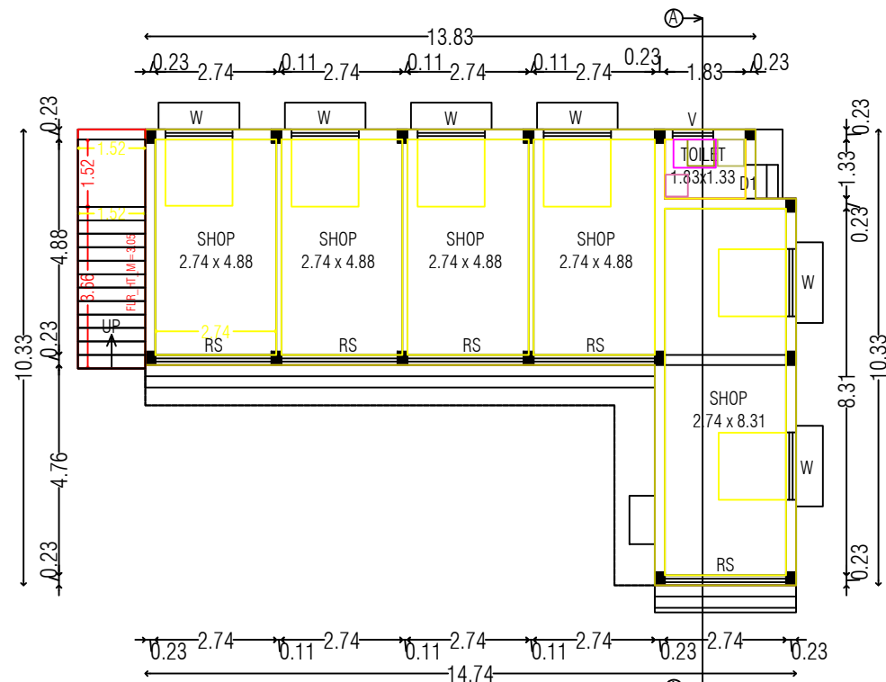
GROUND FLOOR PLAN (WEST FACING) (Scale : - 1:100)
