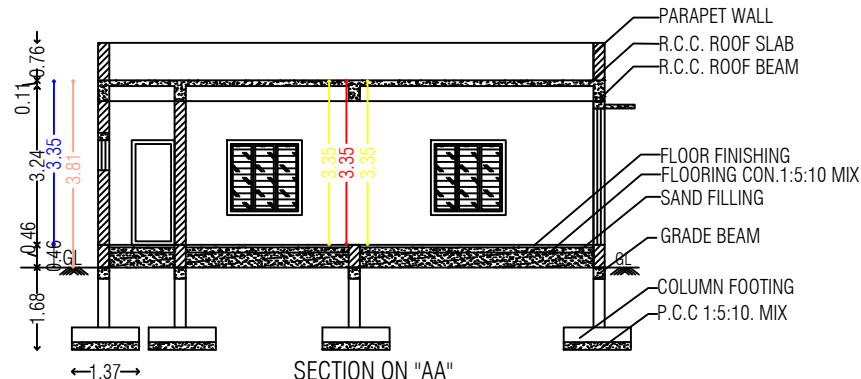
SECTION ON "AA" (Scale : - 1:100)
