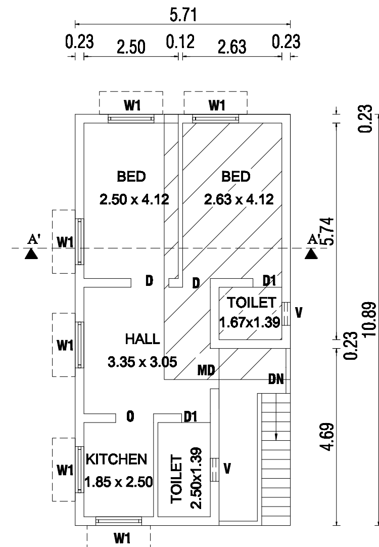
EXISTING & PROPOSED ADDITIONAL FIRST FLOOR PLAN
