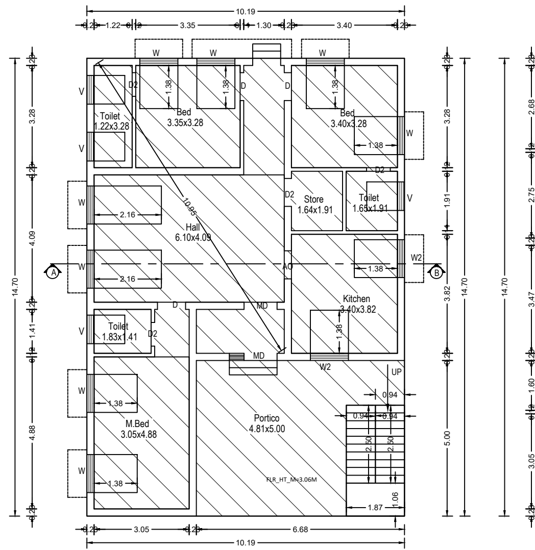
Exg. Ground floor Plan
