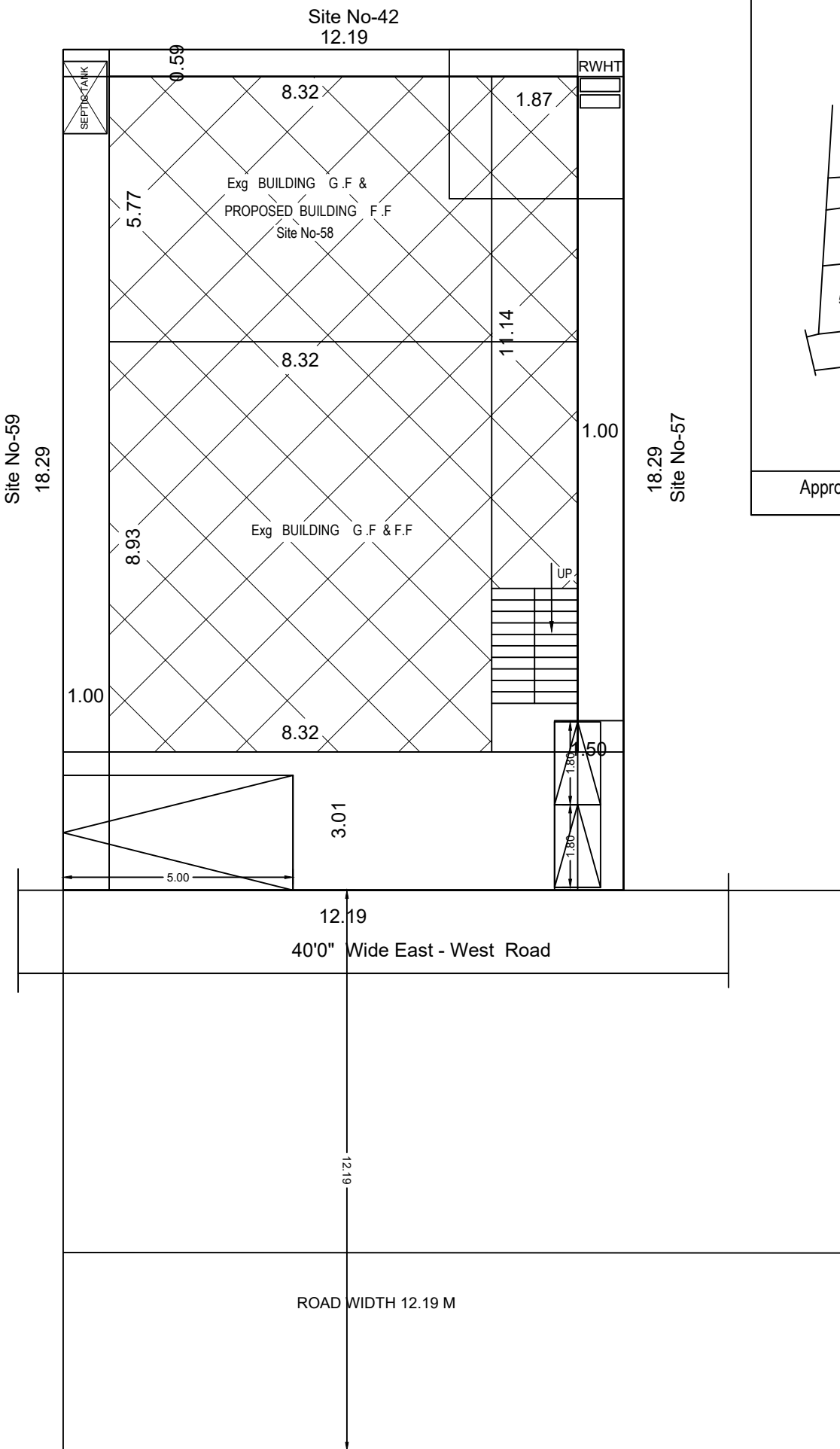
Site Plan
