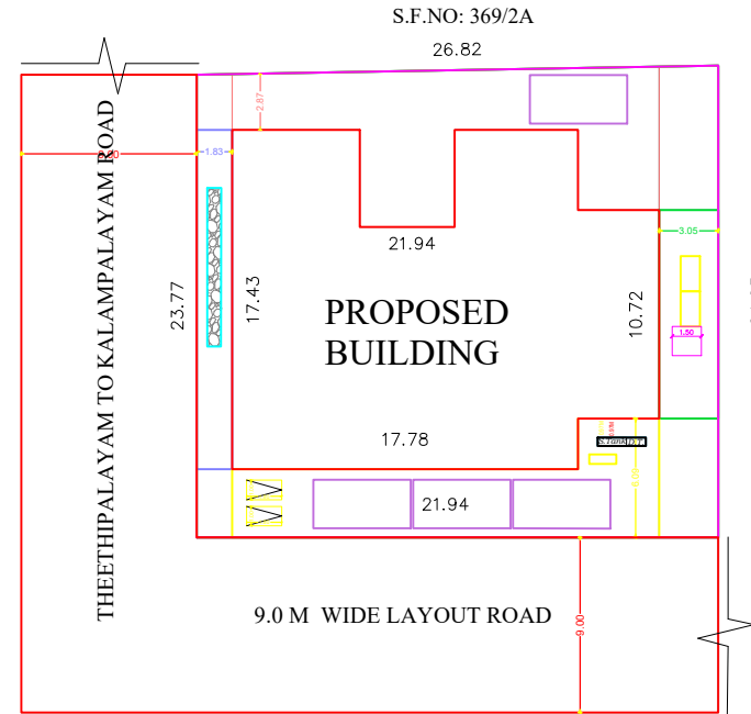
SITE PLAN
