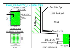
RAIN WATER HARVESTING SYSTEM
