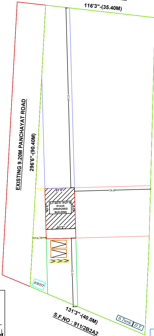
SITE PLAN
