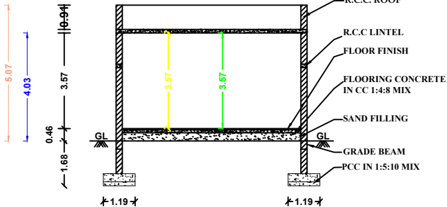
SECTION
