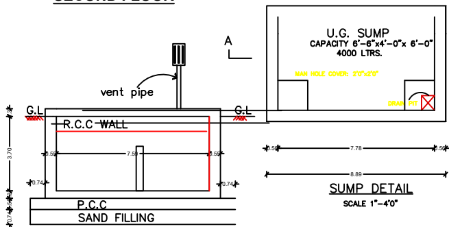
SECTION ON D-D
