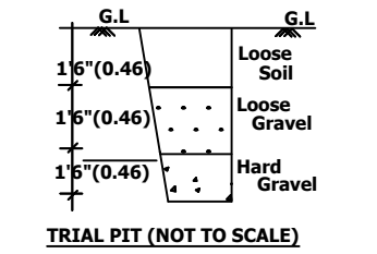
TRIAL PIT (NOT TO SCALE)
