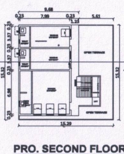
PRO. SECOND FLOOR
