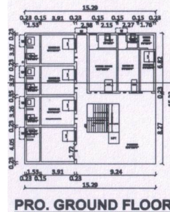
PRO. GROUND FLOOR
