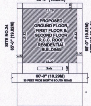
SITE PLAN
