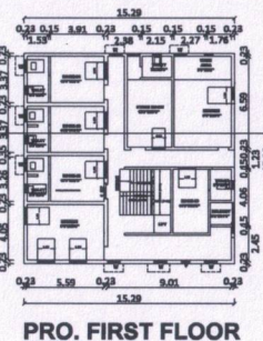
PRO. FIRST FLOOR
