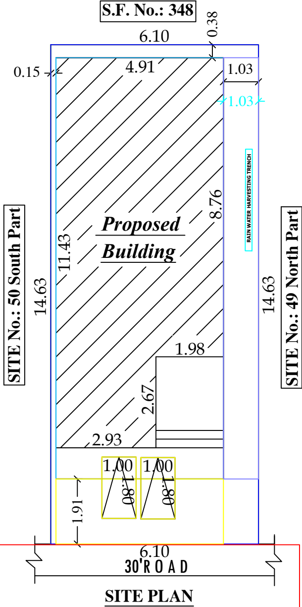
SITE PLAN
