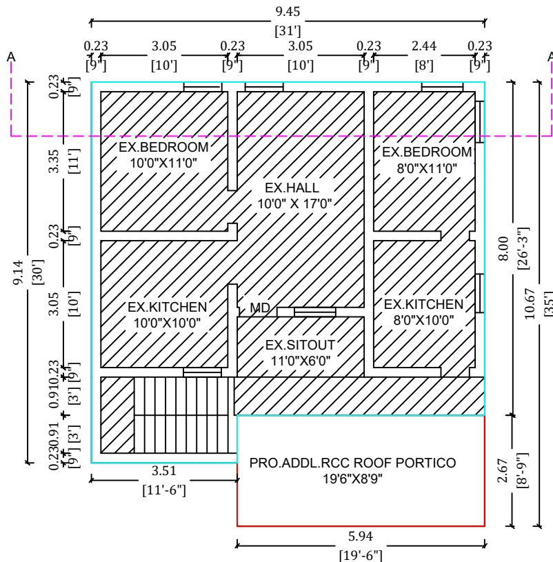
EX.GROUND FLOOR AND PRO.ADDITIONAL GROUND FLOOR R.C.C ROOF PORTICO
