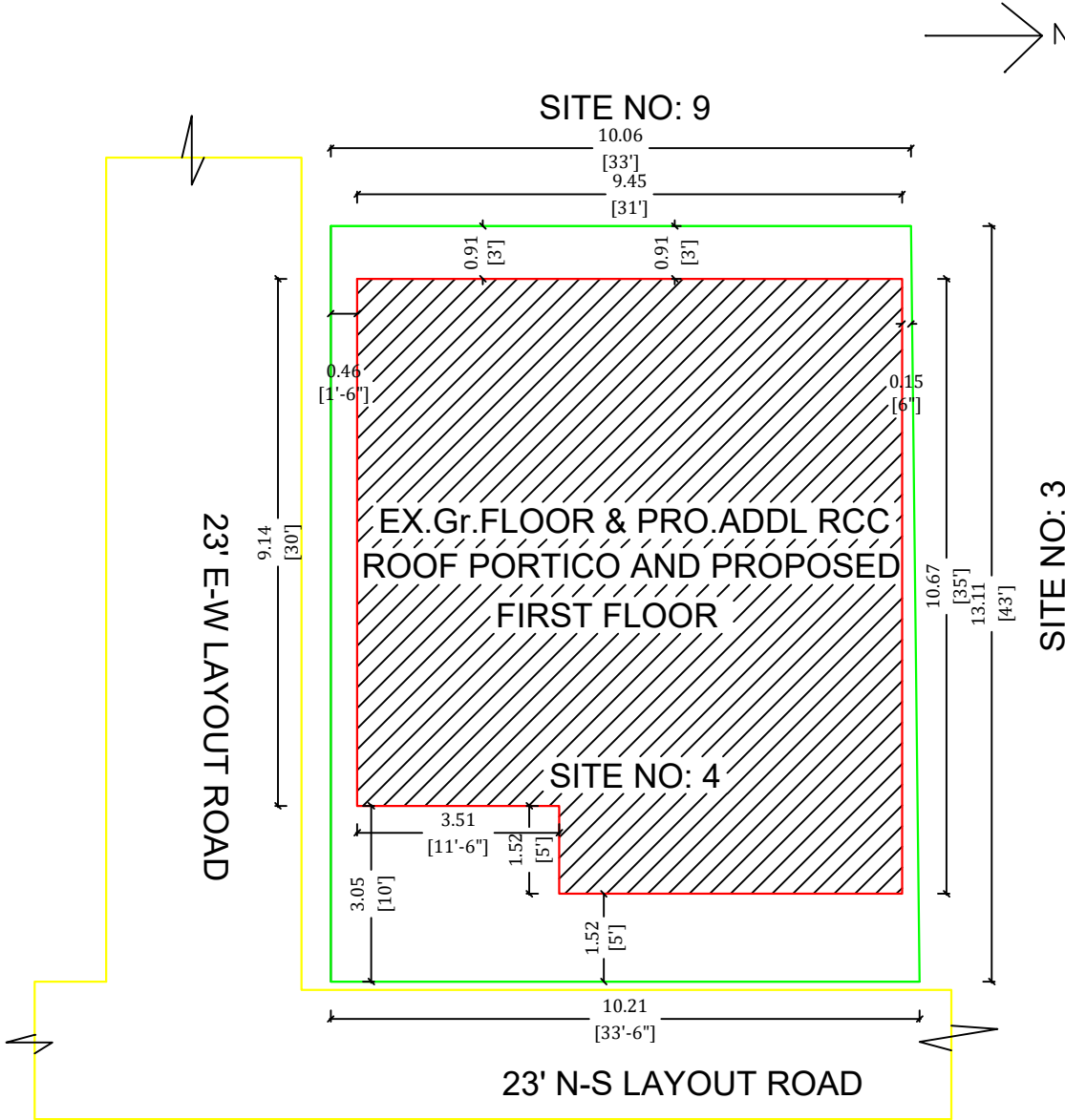
SITE PLAN
