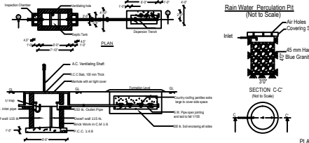
SEPTIC TANK WITH DISPERSION TRENCH ( 250 Gls. ) PLAN
