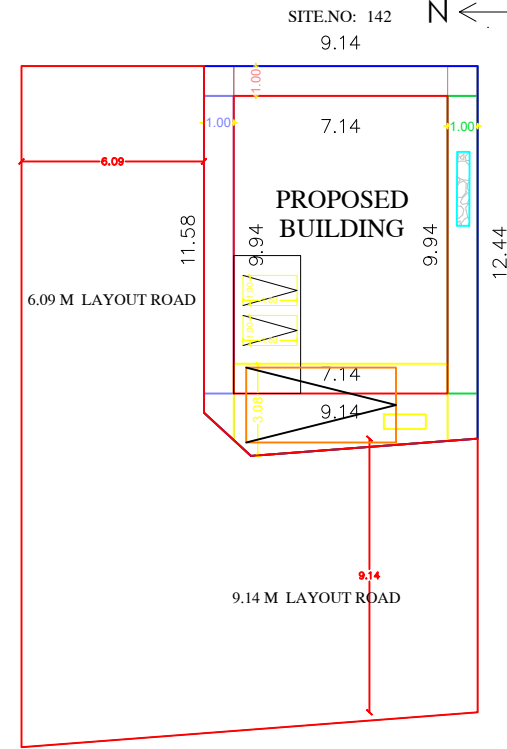
SITE PLAN
