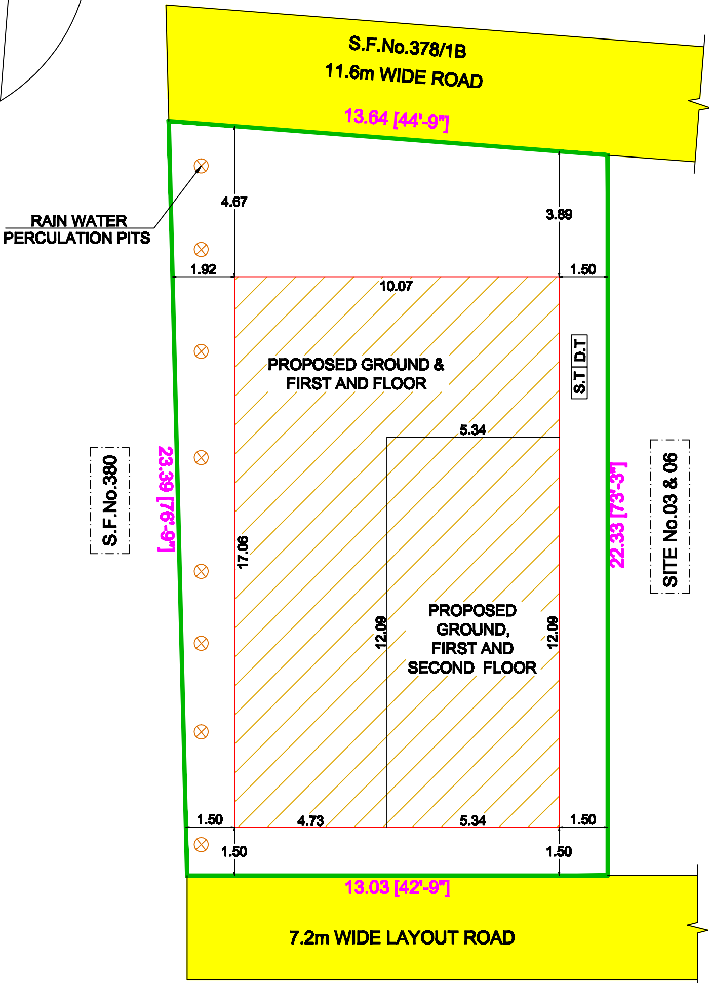
SITE PLAN
