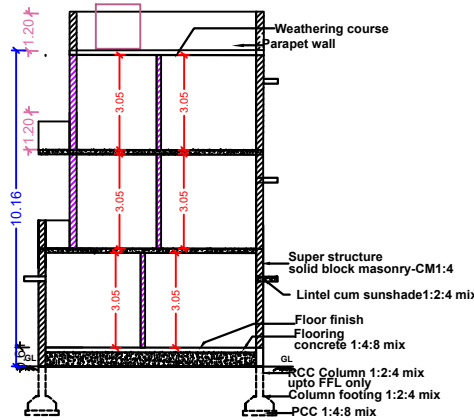
SECTION ELEVATION
