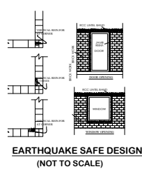
SEISMIC REINFORCEMENT DETAILS (NOT TO SCALE)
