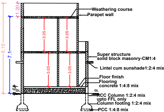
SECTION ELEVATION
