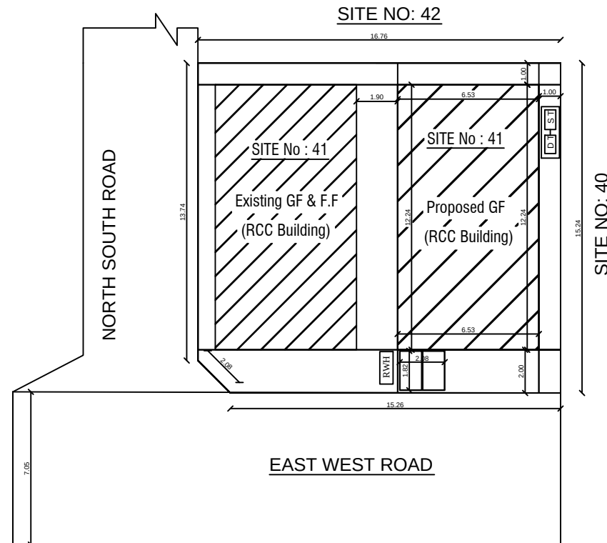
SITE PLAN
