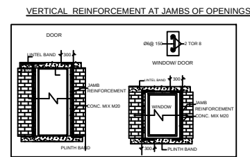
VERTICAL REINFORCEMENT AT JAMBS OF OPENINGS
