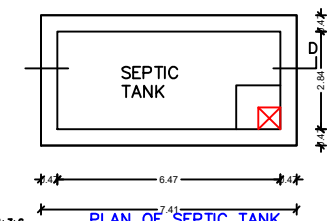
PLAN OF SEPTIC TANK SCALE 1"=2'-0"
