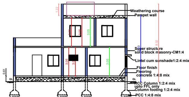
SECTION ELEVATION
