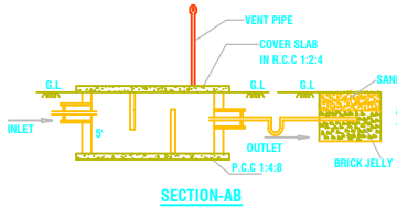
SECTION-AB
