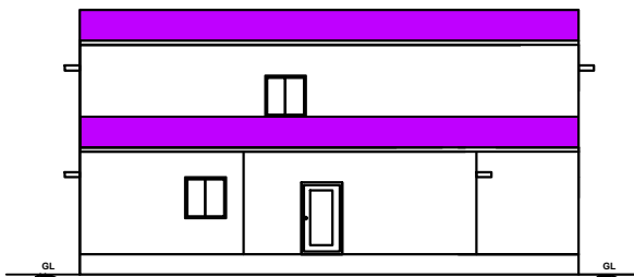
FRONT SIDE ELEVATION
