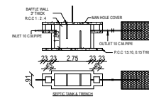
SEPTIC TANK & DRAINAGE
