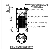
RAIN WATER HARVEST
