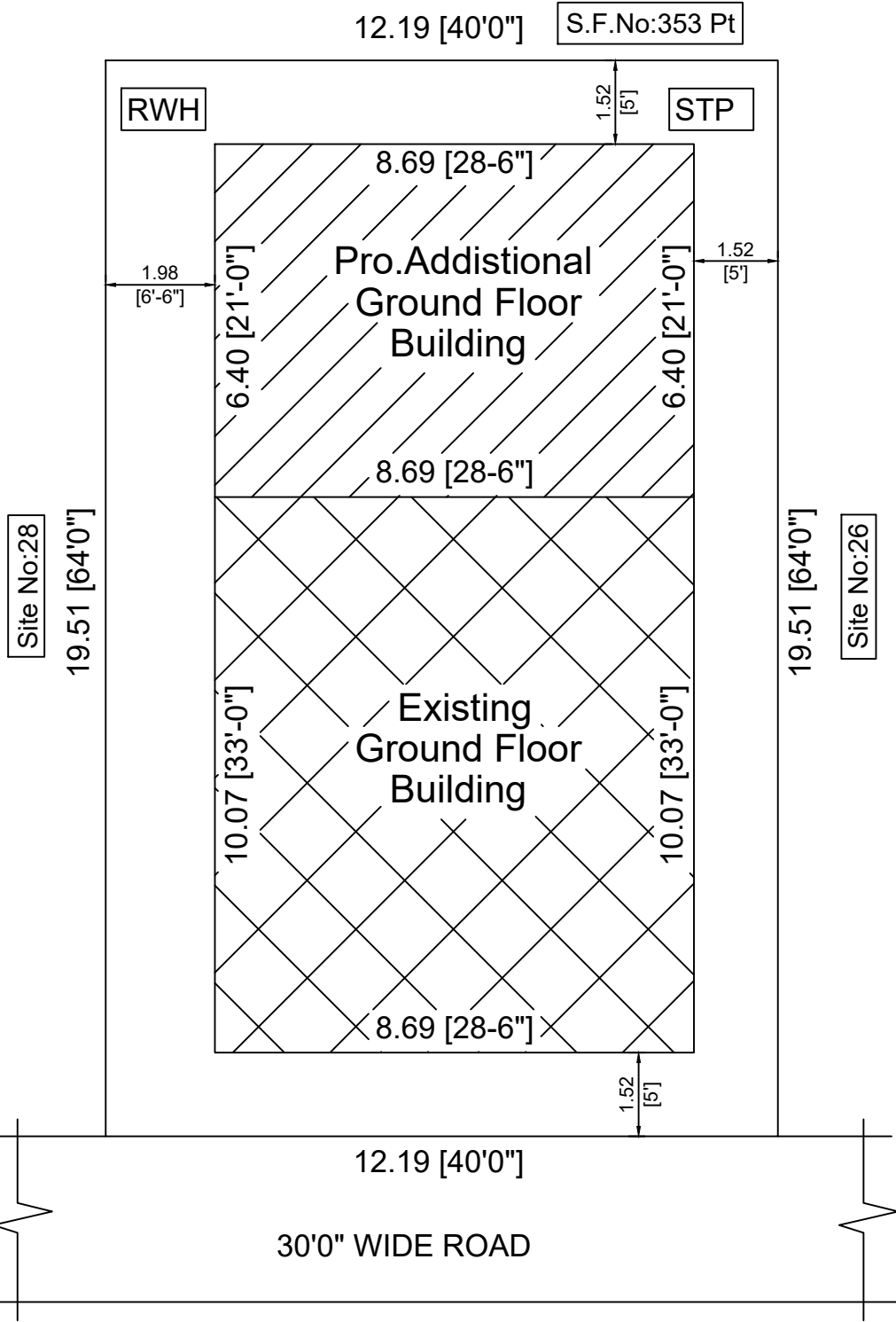
SITE PLAN
