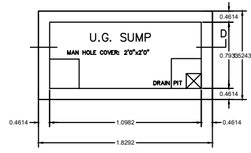
SUMP DETAIL SCALE 1" = 4'0"
