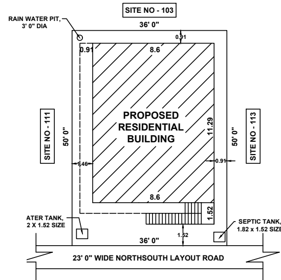
SITE PLAN SCALE - 1' 0" = 10' 0"
