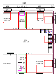
PROPOSED FIRST FLOOR BUILDING
