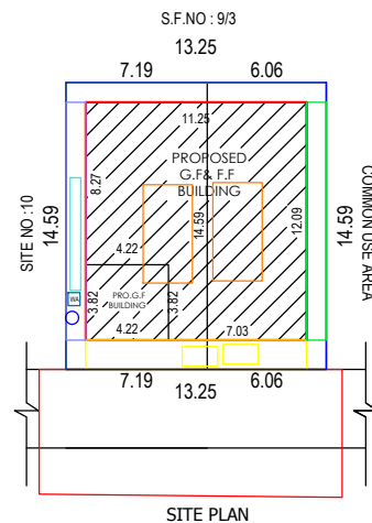
SITE PLAN
