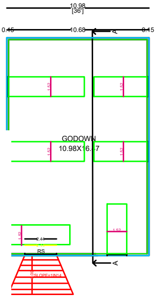
PLAN
