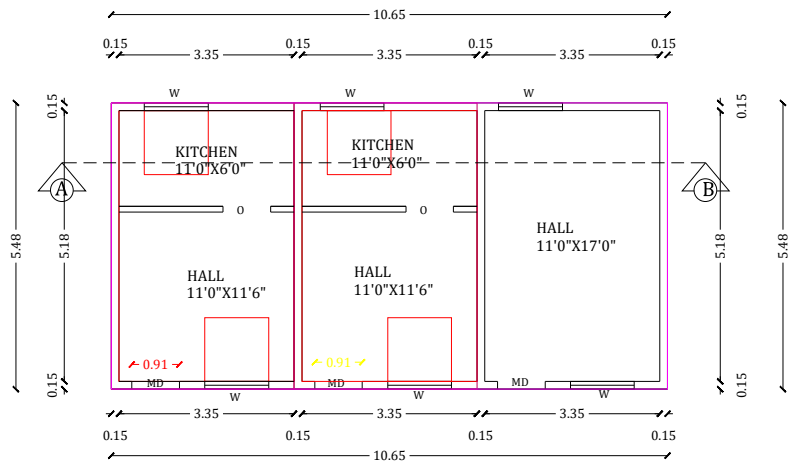
ADD.GROUND FLOOR PLAN
