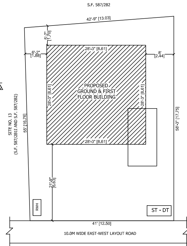
SITE PLAN
