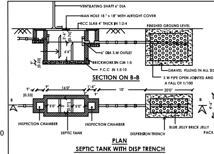
PLAN SEPTIC TANK WITH DISP TRENCH
