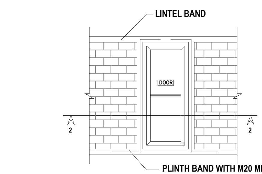
Figure - 3 : Typical Details of Providing Vertical Steel bars in Brick Masonry.
