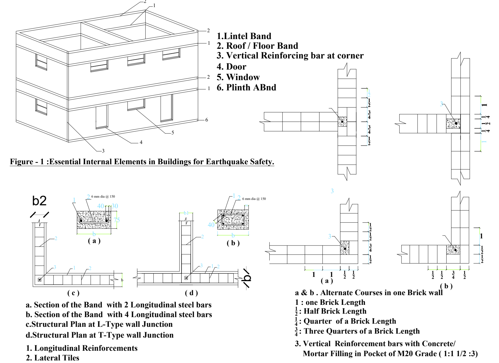
Figure - 1 : Essential Internal Elements in Buildings for Earthquake Safety.
