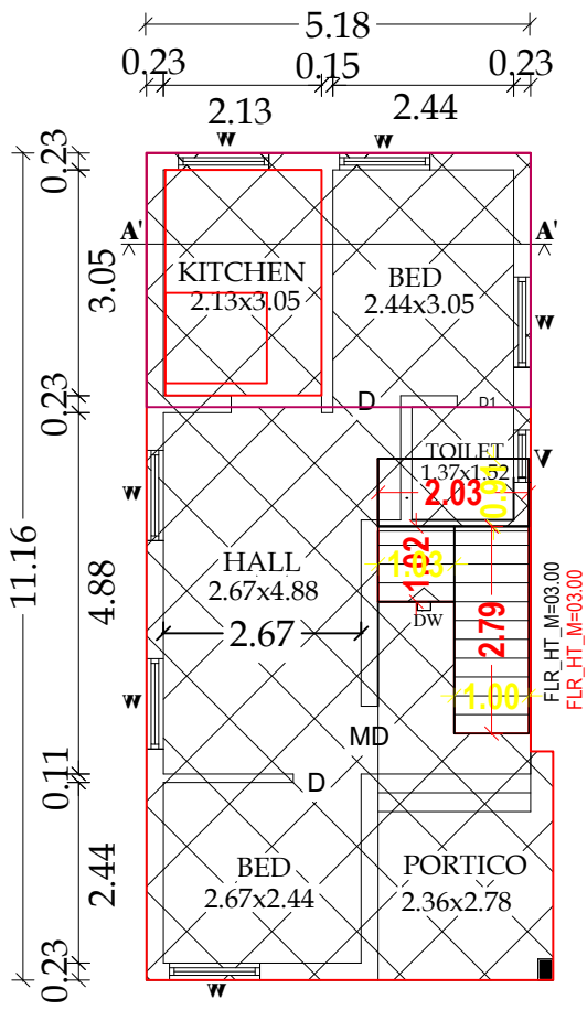
EXI. GROUND FLOOR PLAN
