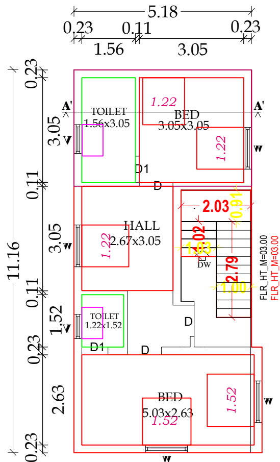
PRO. ADD. FIRST FLOOR PLAN
