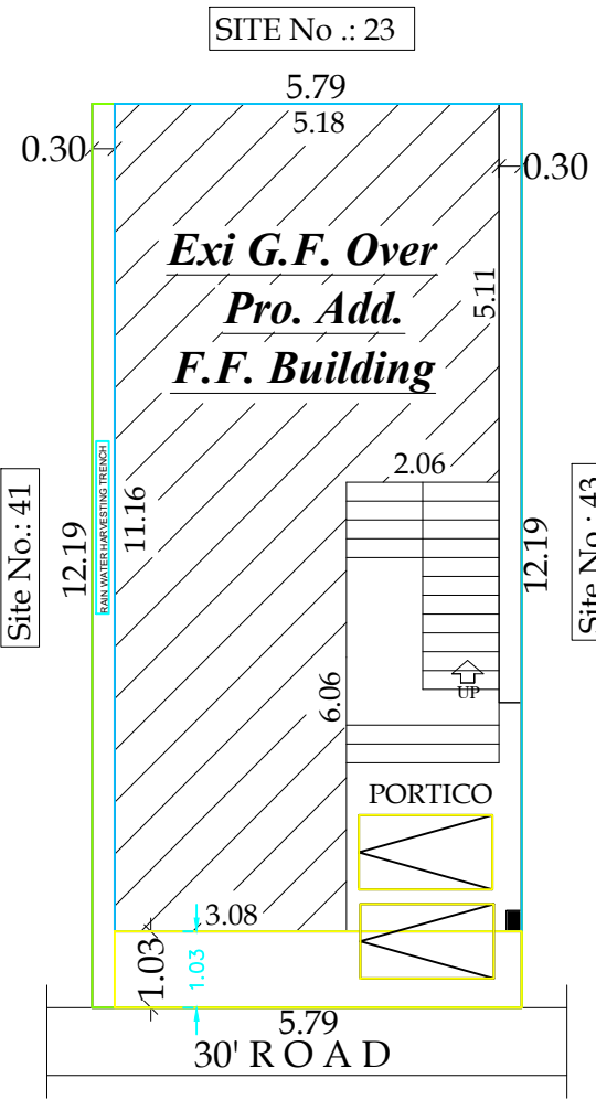
SITE PLAN
