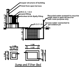
Sump and Filter Bed
