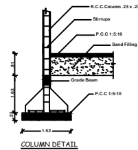
COLUMN DETAIL
