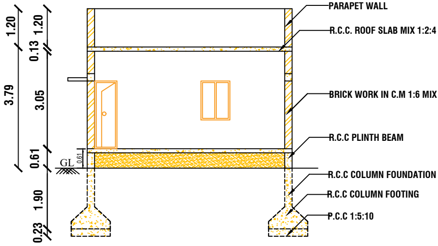
CROSS SECTION AT A-A
