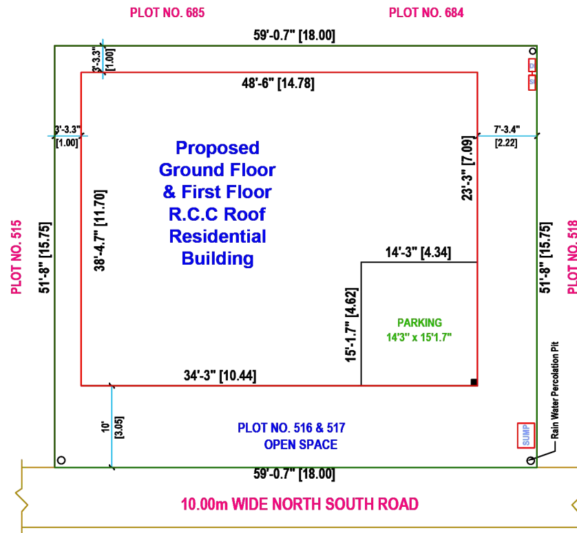
SITE PLAN (SCALE 1" : 8' 0")
