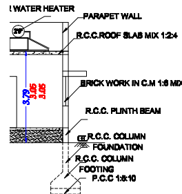
SECTION ON AA'
