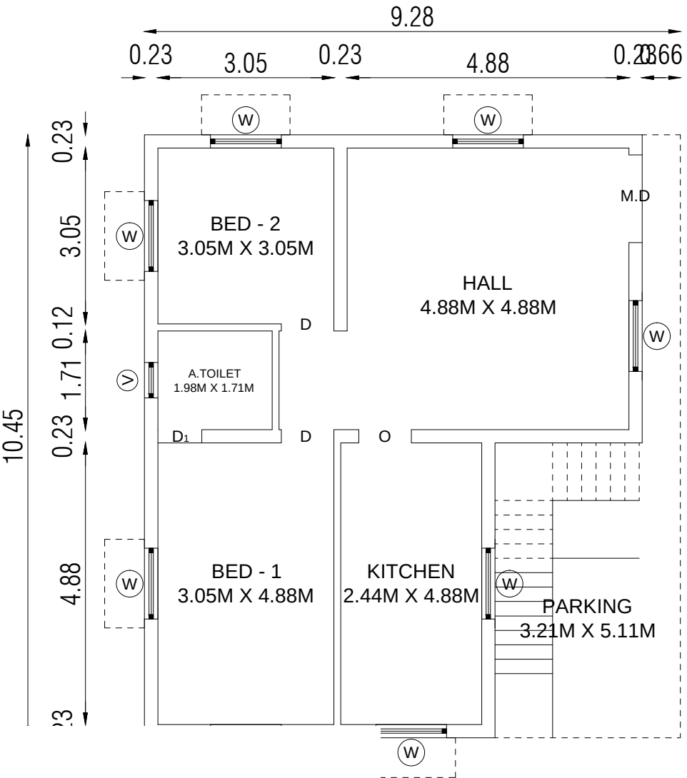
GROUND FLOOR
