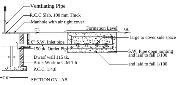
ANK WITH DISPERSION TRENCH ( 250 Gls.)
