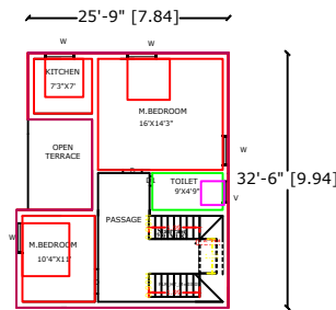
PROPOSED SECOND FLOOR PLAN
